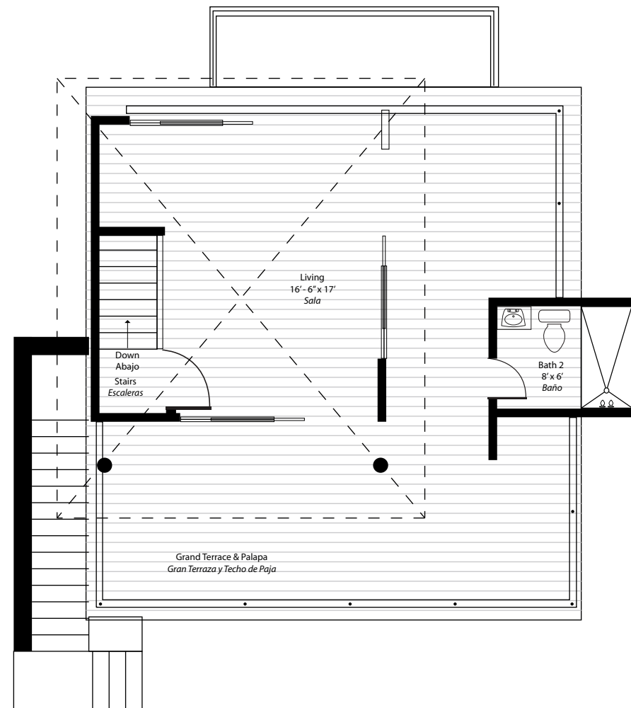
3rd Level 3er Nivel
