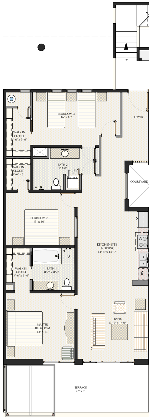
FLOOR PLAN LEVEL 2 - TYPE III
