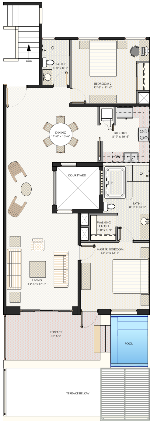
FLOOR PLAN LEVEL 3 - TYPE II
