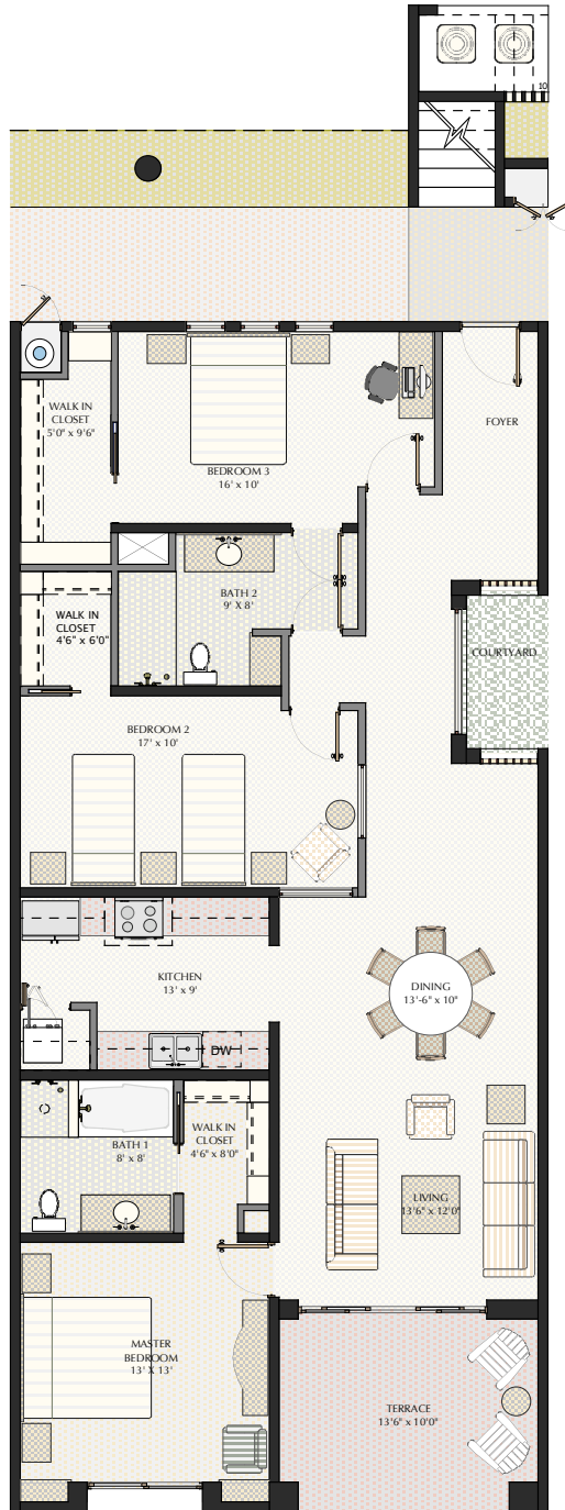
FLOOR PLAN LEVEL 1 - TYPE III
