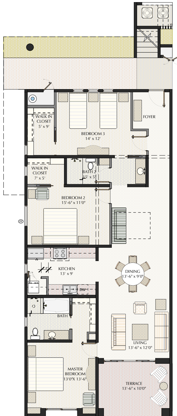
FLOOR PLAN LEVEL 1 - TYPE I
