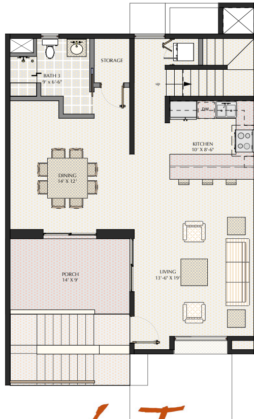
FLOOR PLAN LEVEL 2
